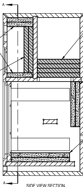
SIDE VIEW SECTION
